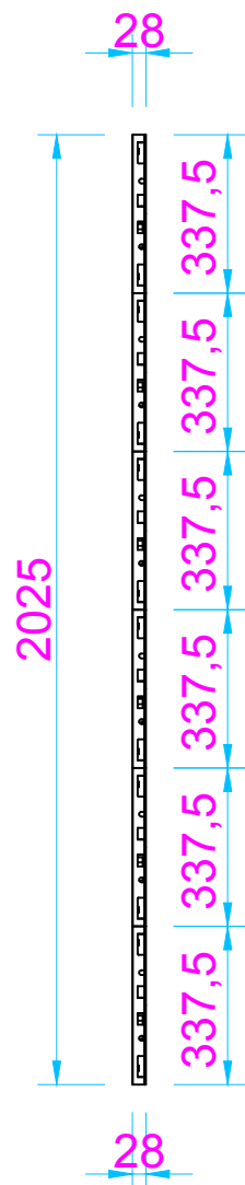
Side view
