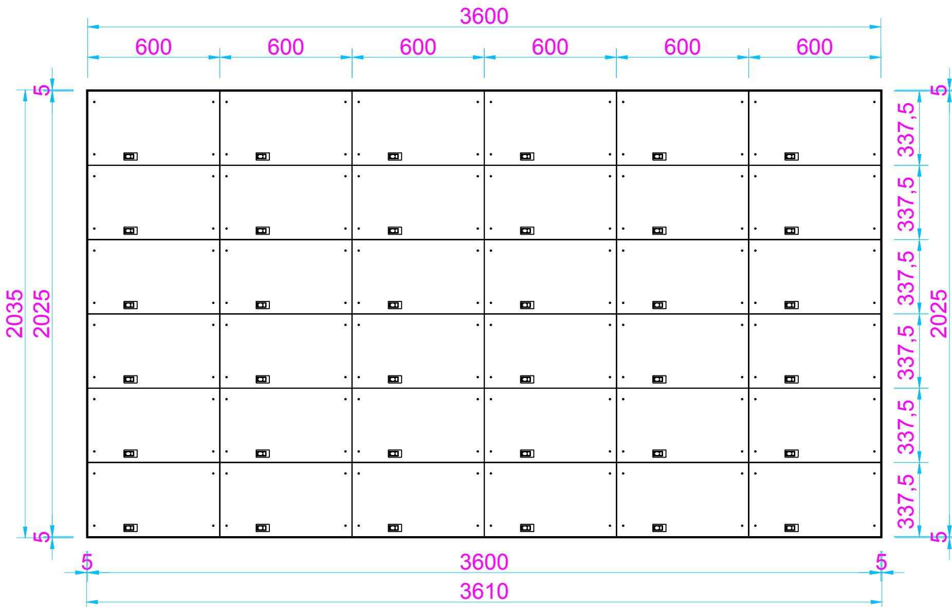
Back view
