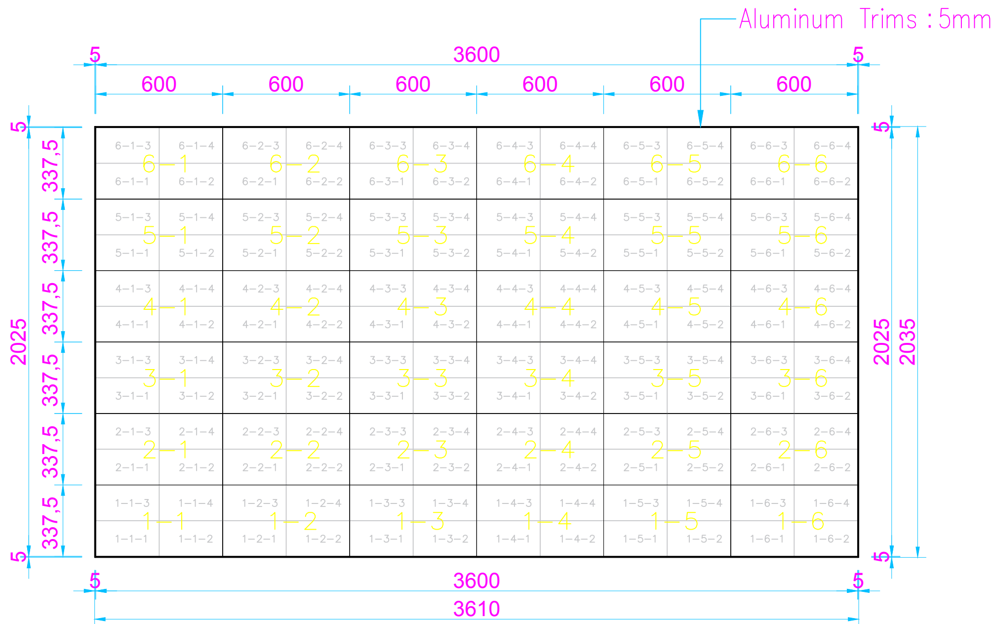
Front view
